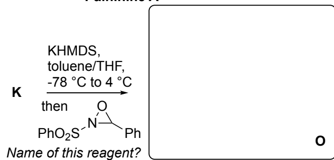
Palhinine A
