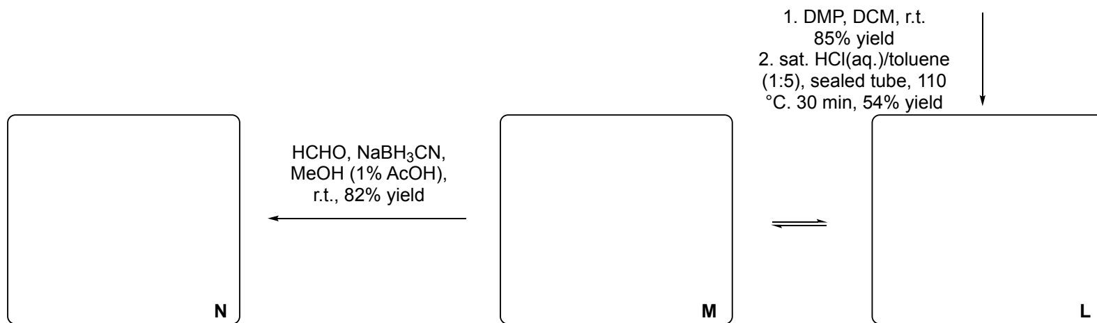
Palhinine A
