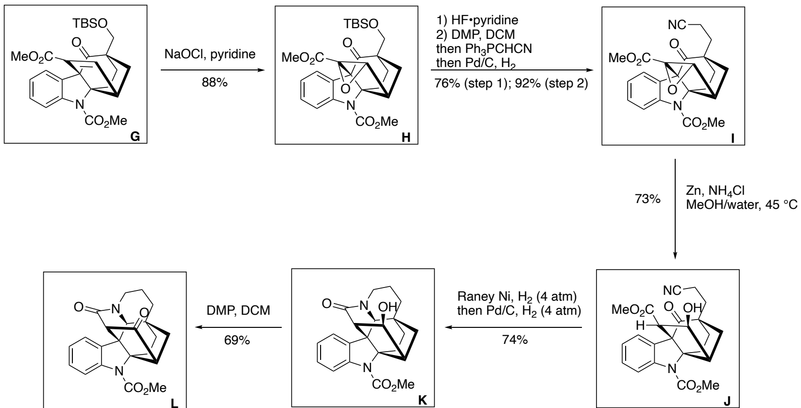
N - Carbomethoxy-10,22- dioxokopsane
